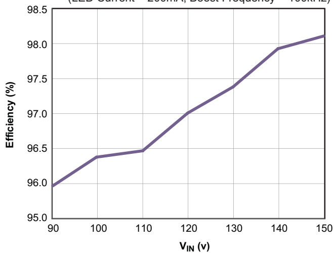
Efficiency vs. V_{IN} @ OUT = 195V
