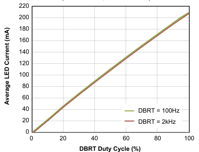
DBRT Control Linearity
