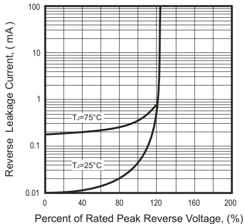
Fig.5- Reverse Characteristics
