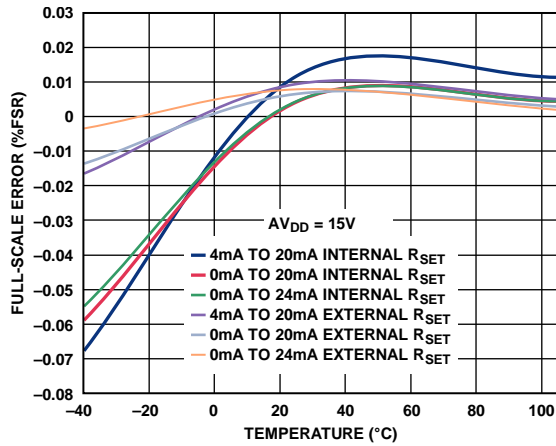
Figure 16. Full-Scale Error vs. Temperature
