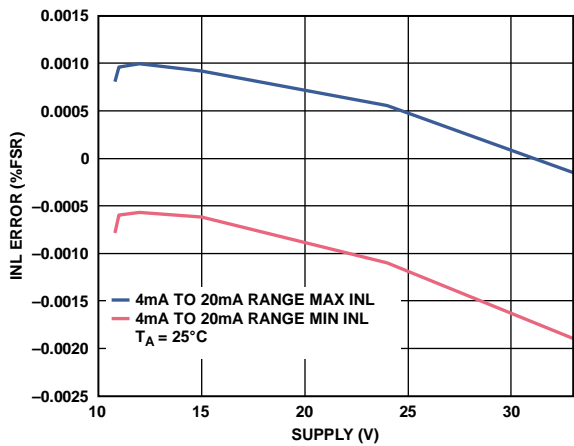
Figure 20. Integral Nonlinearity Error vs. AV_{DD} , Over Supply, Internal R_{SET}
