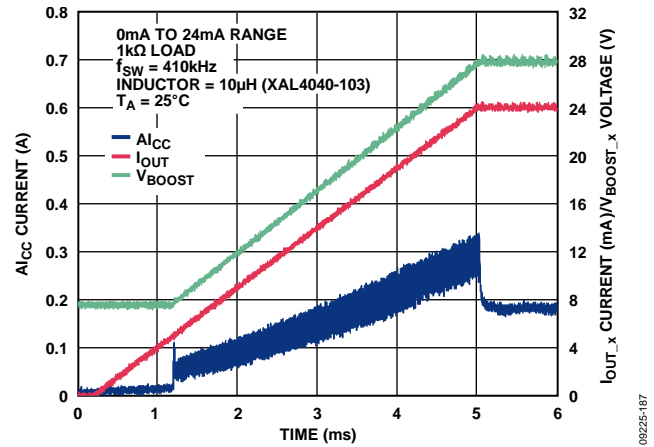
Figure 62. I_{CC} Current vs. Time for 24 mA Step Through 1 k \Omega Load with Slew Rate Control
