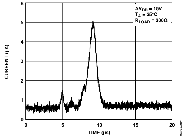
Figure 25. Output Current vs. Time on Power-Up
