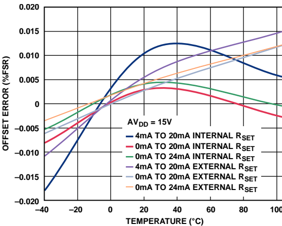
Figure 17. Offset Error vs. Temperature
