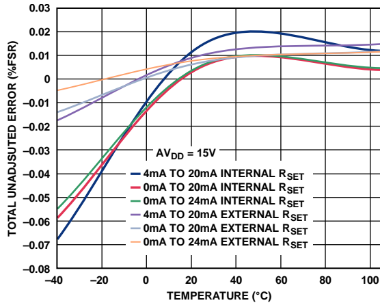
Figure 15. Total Unadjusted Error vs. Temperature
