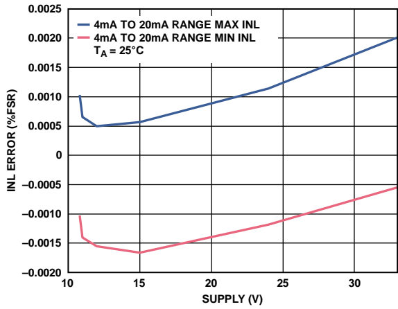
Figure 19. Integral Nonlinearity Error vs. AV_{DD} , Over Supply, External R_{SET}
