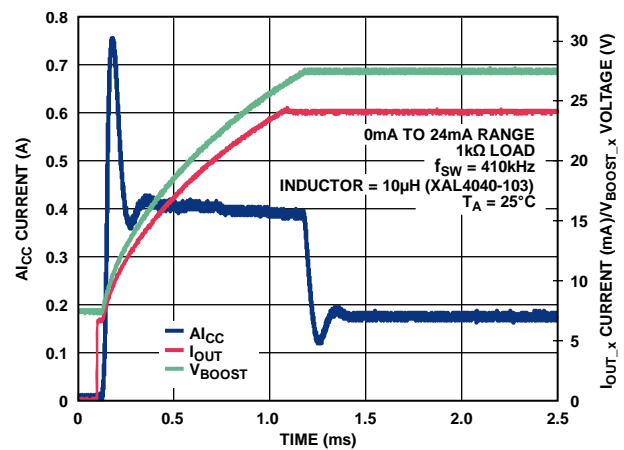
Figure 59. AI_{\text{CC}} Current vs. Time for 24 mA Step Through 1 k \Omega Load with Internal Compensation Resistor
