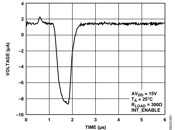
Figure 26. Output Current vs. Time on Output Enable
