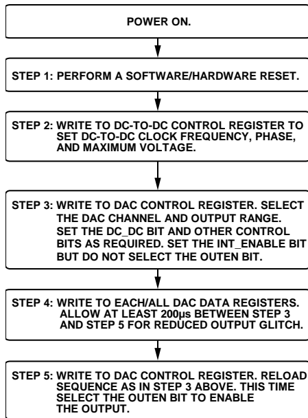
Figure 52. Programming Sequence for Enabling the Output Correctly
