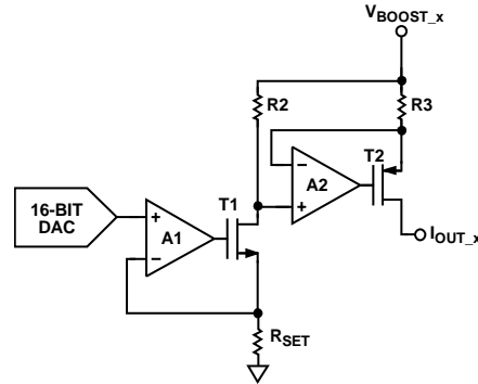
Figure 73. Voltage-to-Current Conversion Circuitry
