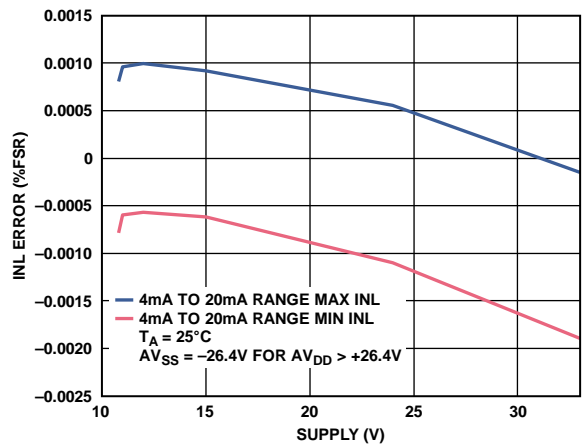
Figure 43. Integral Nonlinearity Error vs. AV_{DD}/|AV_{SS}| , Over Supply, Internal R_{SET}
