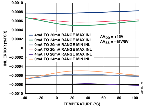
Figure 36. Integral Nonlinearity vs. Temperature, Internal RSET
