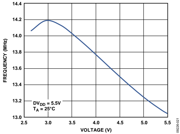
Figure 71. Internal Oscillator Frequency vs. DV DD Supply Voltage
