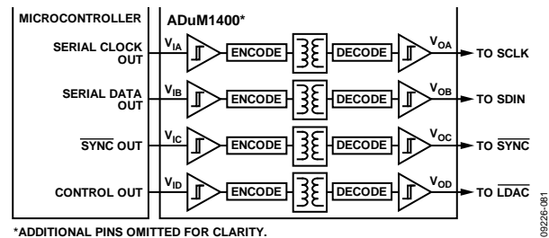
Figure 89. Isolated Interface
