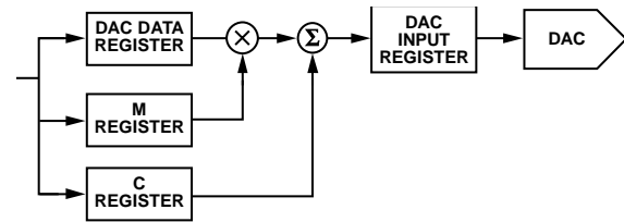
Figure 78. Digital Offset and Gain Control
