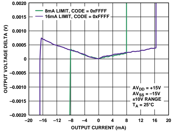
Figure 24. Source and Sink Capability of Output Amplifier
