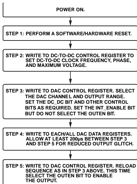
Figure 76. Programming Sequence for Enabling the Output Correctly
