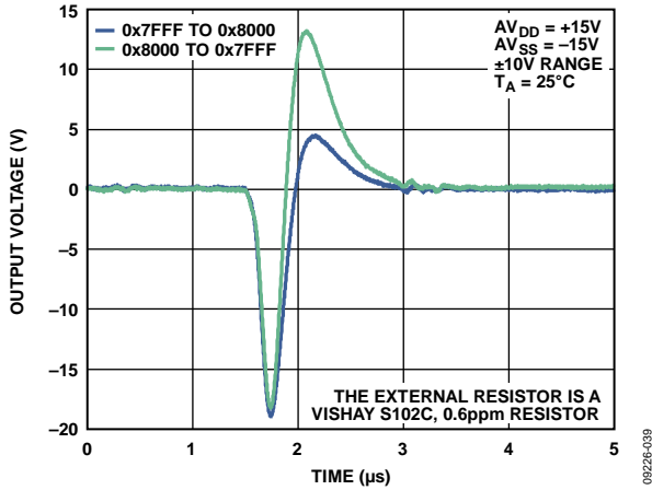
Figure 27. Digital-to-Analog Glitch
