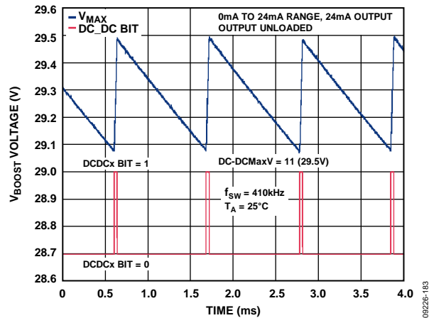
Figure 82. Operation on Reaching V MAX
