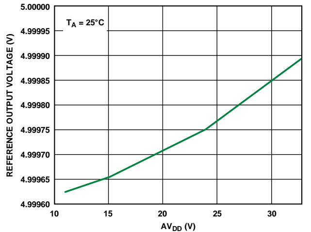
Figure 66. REFOUT vs. Supply
