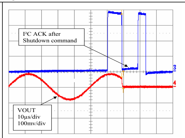
Figure 71. Shutdown time
