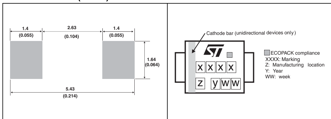
Figure 17. SMA footprint dimensions in mm (inches)
