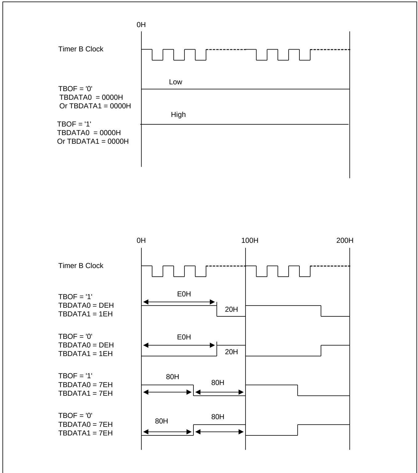
Figure 13-15 Timer B Output Flip-Flop Waveforms in Repeat Mode
