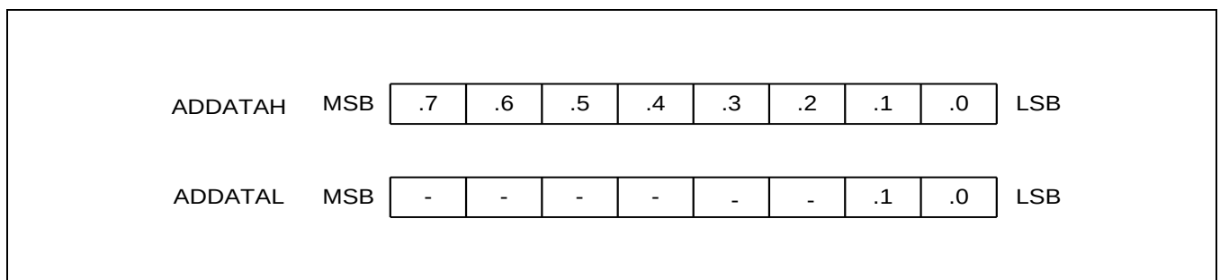
Figure 16-3 A/D Converter Data Register (ADDATAH/L)
