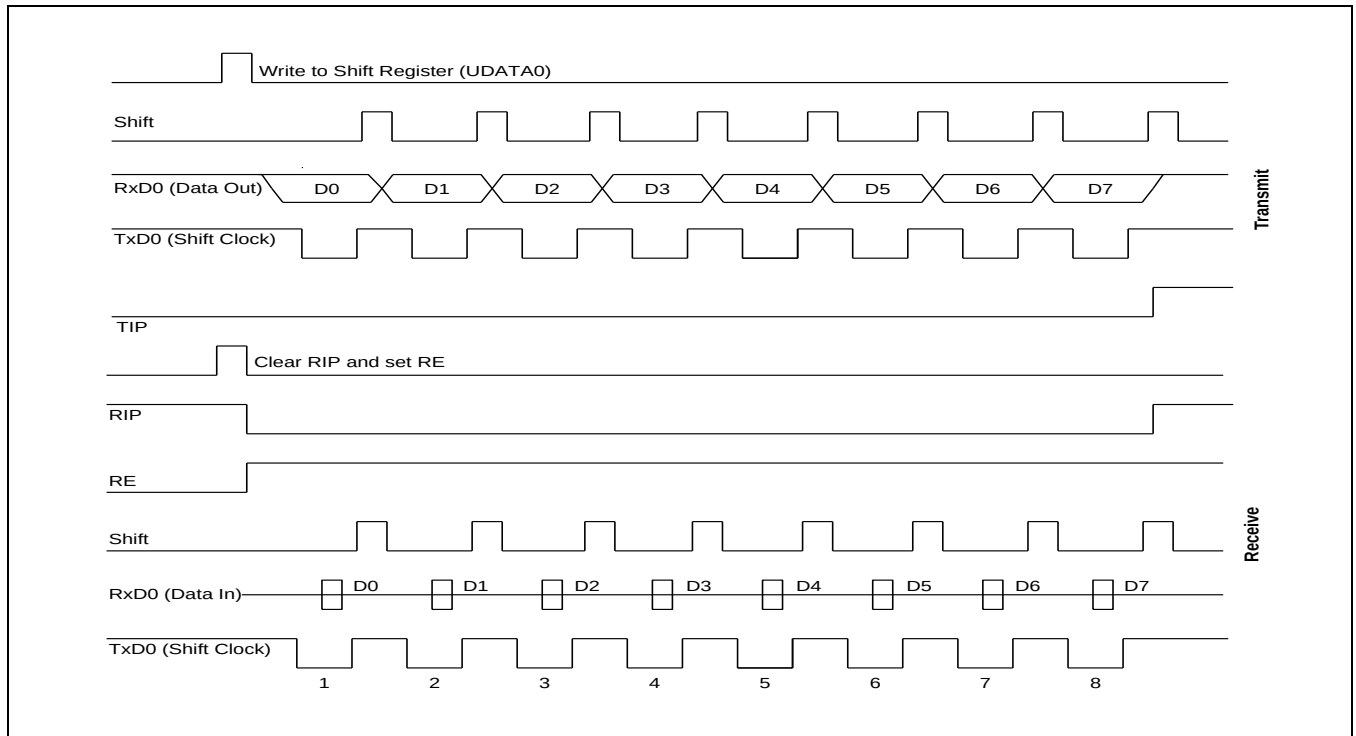
Figure 19-6 Timing Diagram for Serial Port Mode 0 Operation
