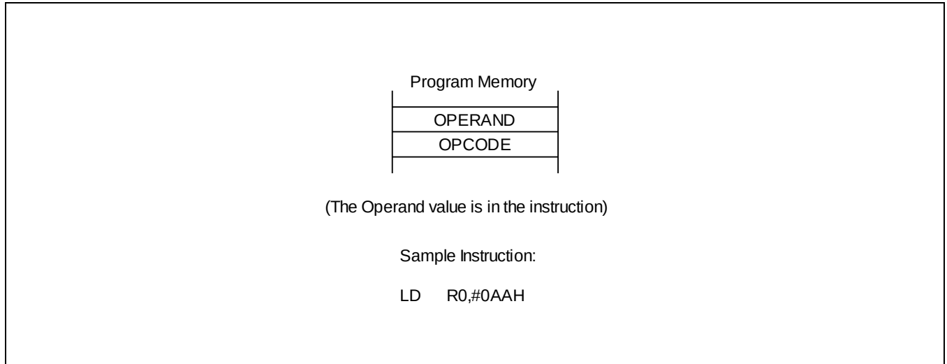
Figure 3-14 Immediate Addressing
