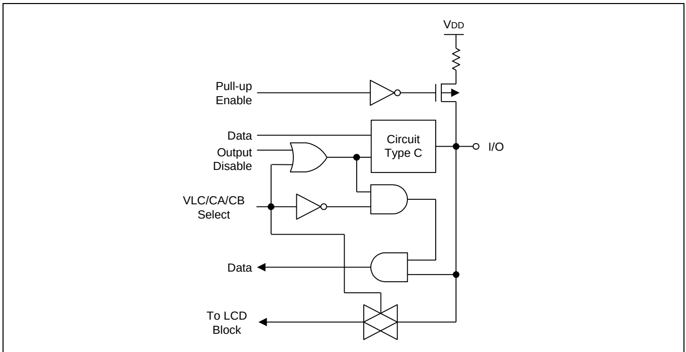
Figure 1-9 Pin Circuit Type F-17(P1)
