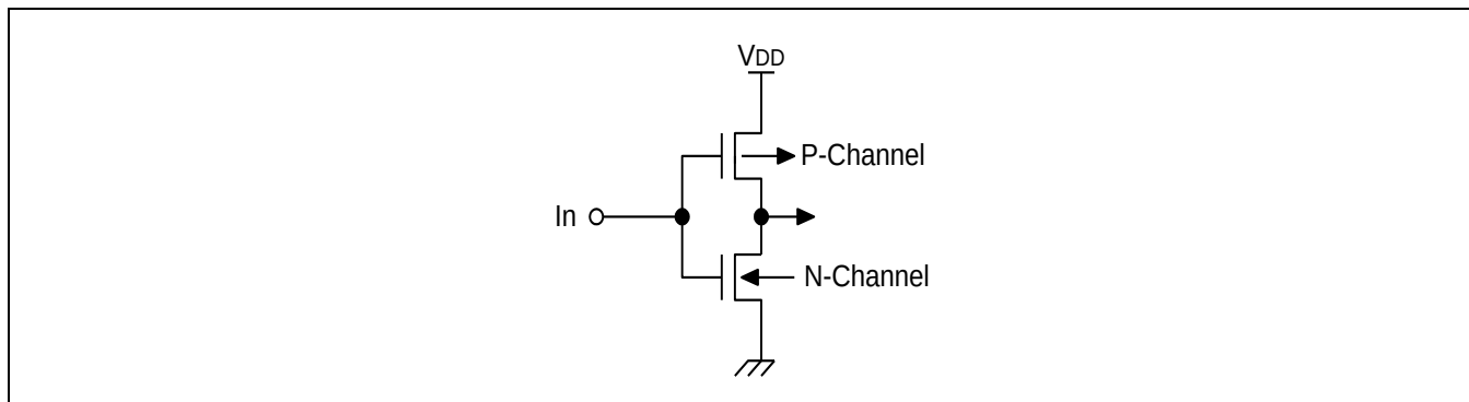
Figure 1-3 Pin Circuit Type A
