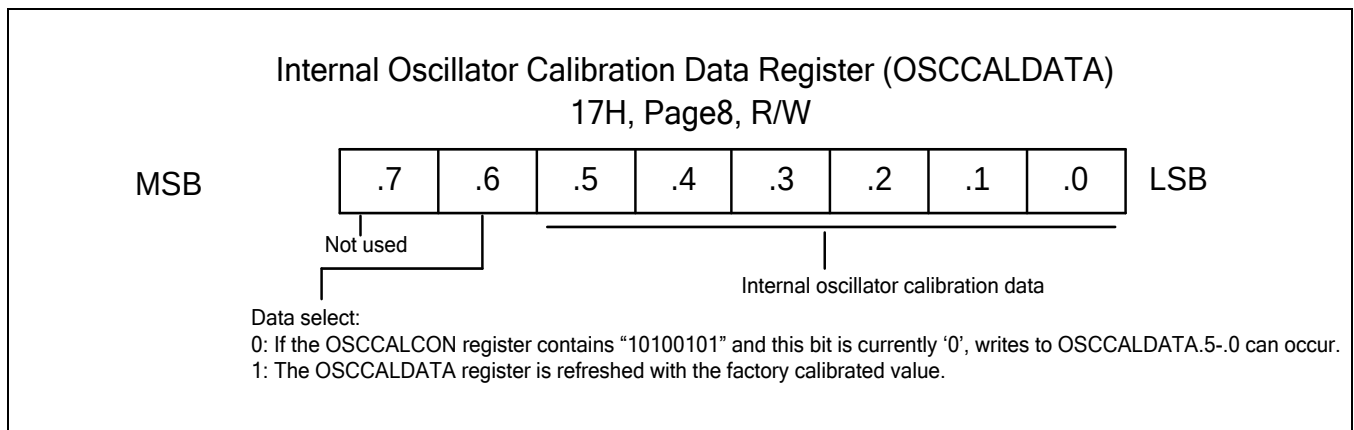
Figure 7-6 Internal Oscillator Calibration Data Register (OSCCALDATA)
