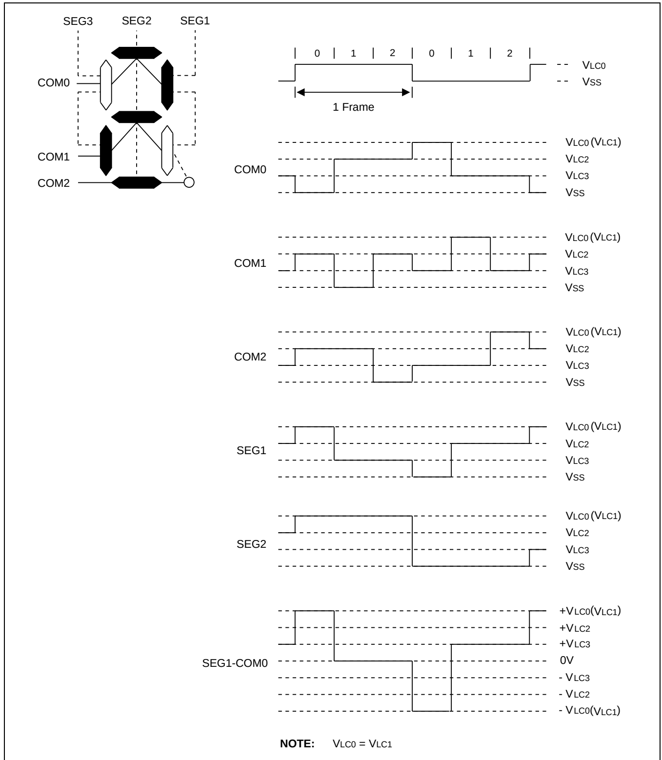
Figure 15-12 LCD Signal Waveforms (1/3 Duty, 1/3 Bias)
