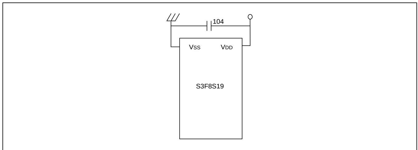
Figure 23-6 The Circuit Diagram to Improve EFT Characteristics
