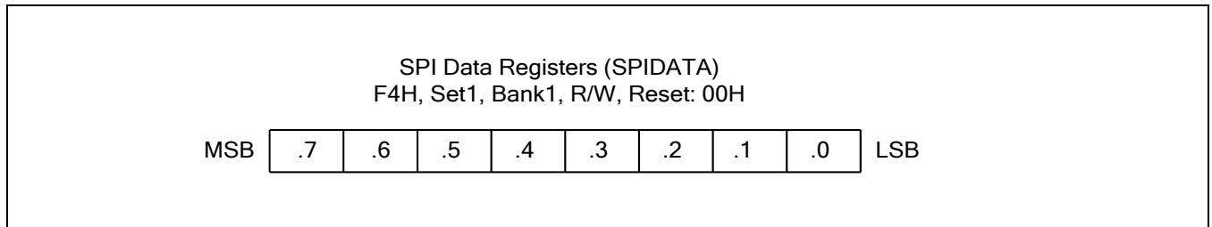
Figure 17-5 SPI Data Register (SPIDATA)
