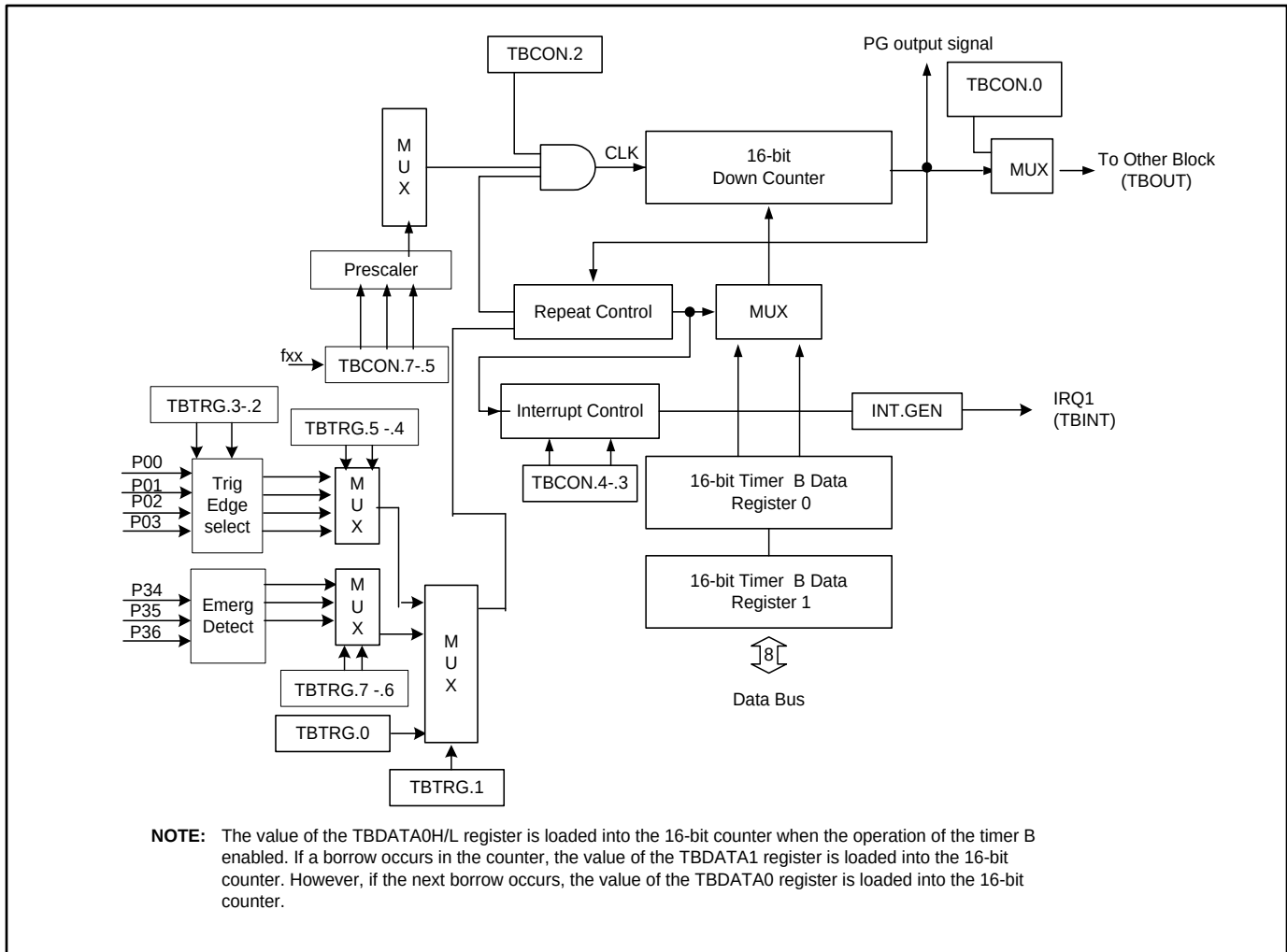
Figure 13-14 Timer B Functional Block Diagram
