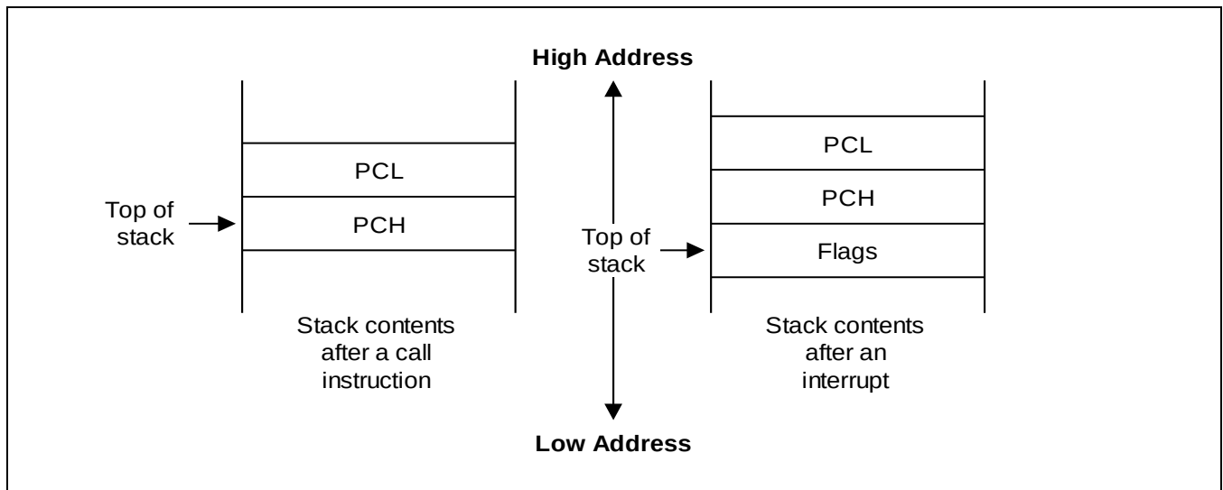
Figure 2-16 Stack Operations
