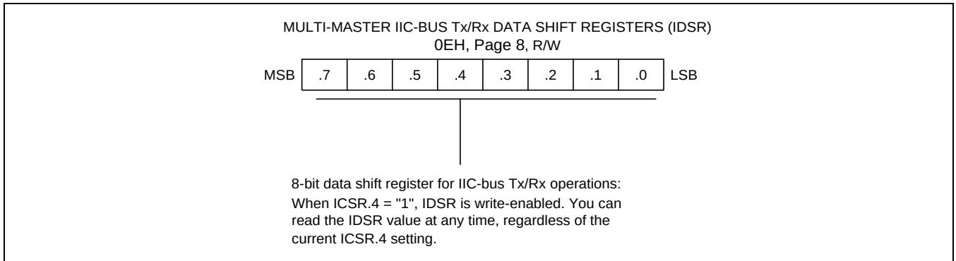
Figure 18-3 Multi-Master I2C Bus Tx/Rx Data Shift Register (IDSR)
