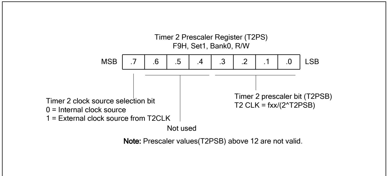
Figure 13-8 Timer 2 Prescaler Register (T2PS)
