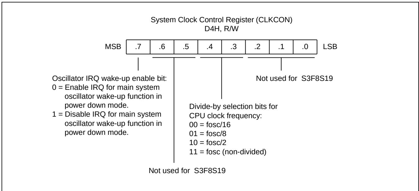
Figure 7-4 System Clock Control Register (CLKCON)
