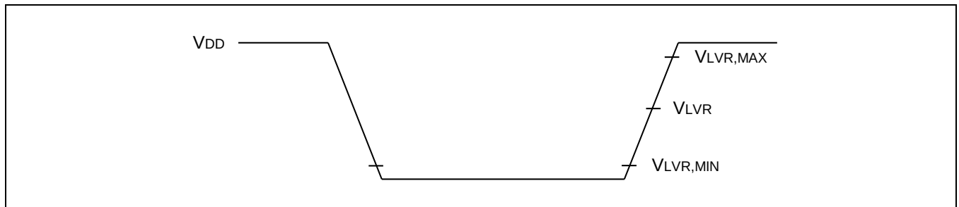
Figure 23-5 LVR Reset Timing
