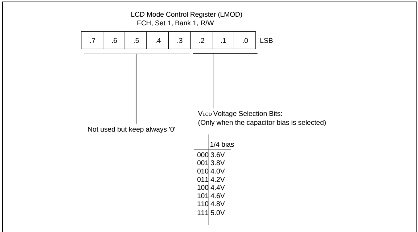
Figure 15-5 LCD Mode Control Register (LMOD)
