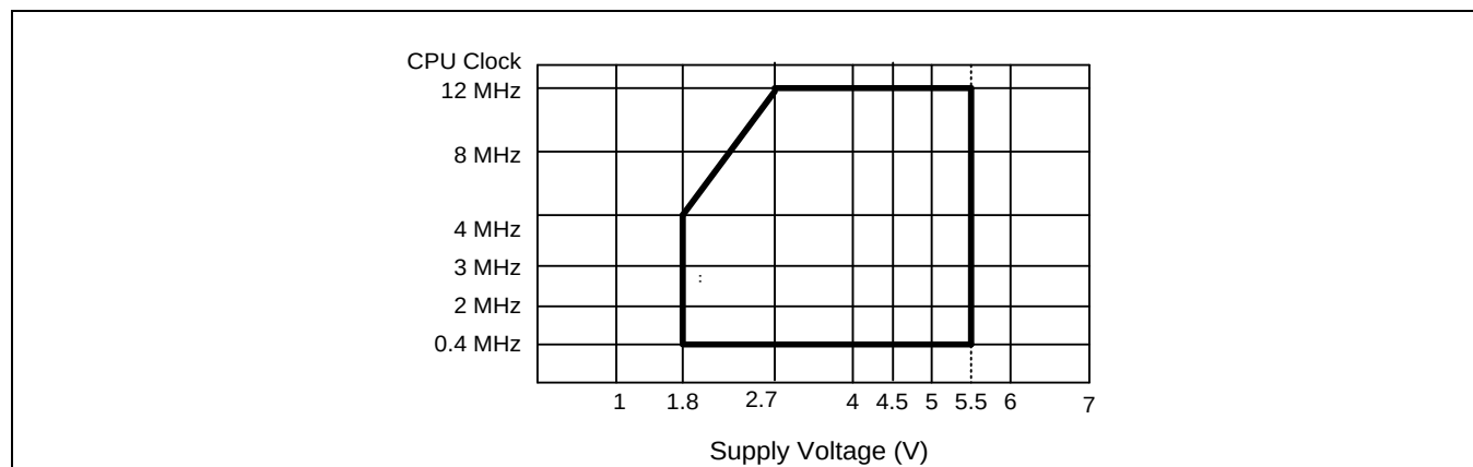
Figure 23-2 Operating Voltage Range
