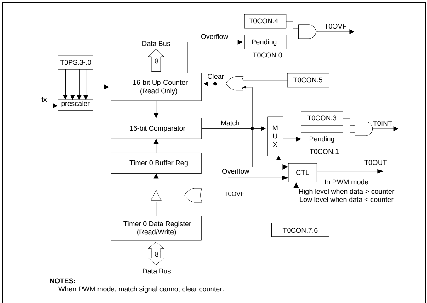
Figure 13-3 Timer 0 Functional Block Diagram
