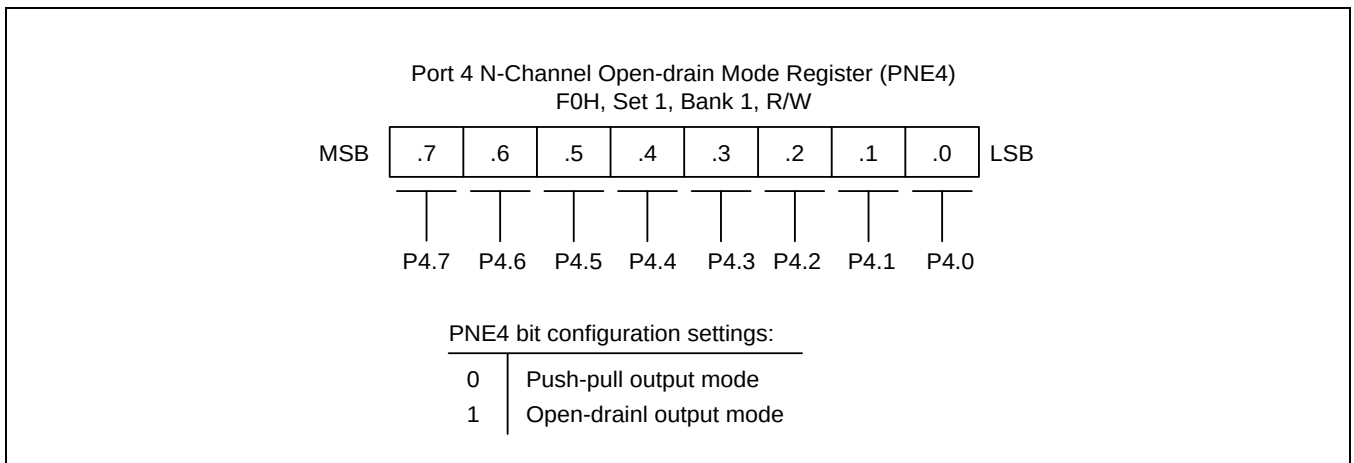
Figure 9-17 Port 4 N-Channel Open-Drain Mode Register (PNE4)
