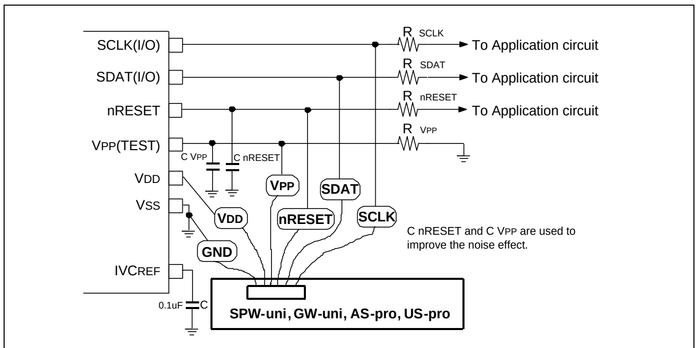
Figure 25-3 PCB Design Guide for on Board Programming
