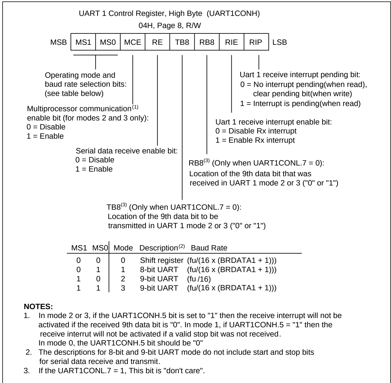
Figure 20-1 UART 1 High Byte Control Register (UART1CONH)
