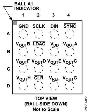
Figure 6. 16-Ball WLCSP (CB-16-16)
