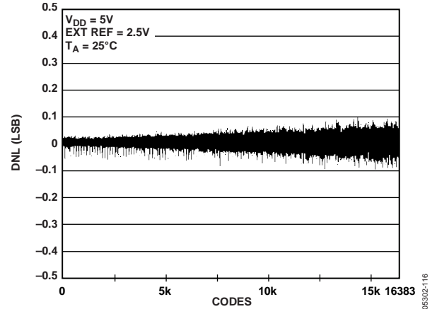
Figure 17. DNL AD5648-2
