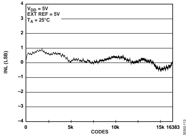
Figure 14. INL AD5648-2
