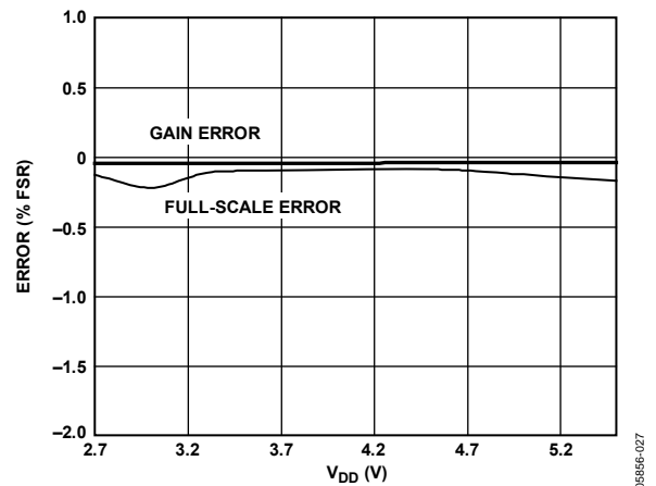
Figure 28. Gain Error and Full-Scale Error vs. Supply
