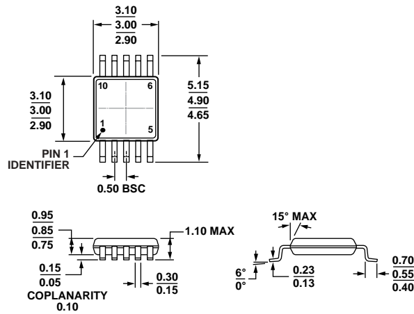
COMPLIANT TO JEDEC STANDARDS MO-187-BA Figure 66. 10-Lead Mini Small Outline Package [MSOP] (RM-10) Dimensions shown in millimeters
