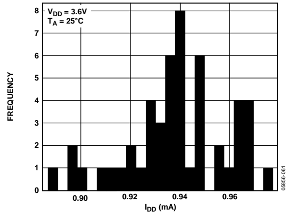
Figure 33. I_{DD} Histogram with Internal Reference, V_{REFOUT} = 1.25 V
