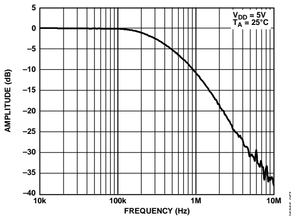
Figure 50. Multiplying Bandwidth
