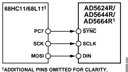
Figure 59. 68HC11/68L11 Interface to AD5624R/AD5644R/AD5664R
