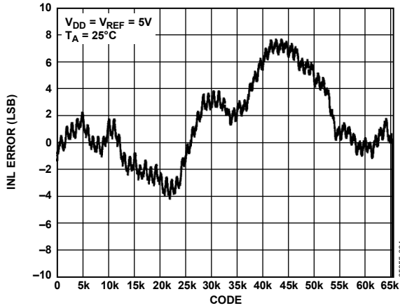
Figure 5. INL
