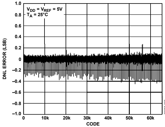
Figure 6. DNL
