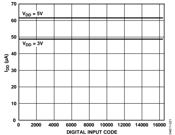
Figure 22. Supply Current vs. Digital Input Code
