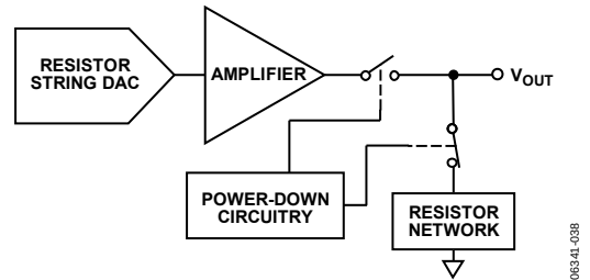
Figure 70. Output Stage During Power-Down
