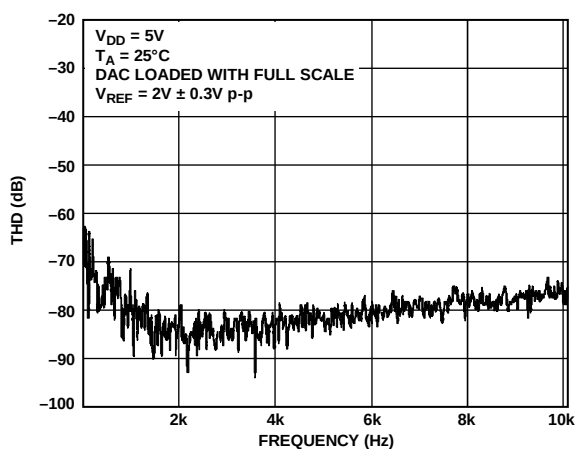
Figure 52. Total Harmonic Distortion
