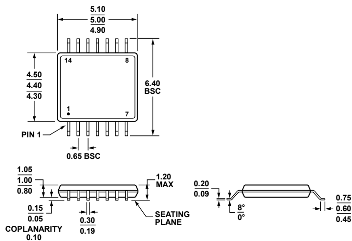
COMPLIANT TO JEDEC STANDARDS MO-153-AB-1 Figure 77. 14-Lead Thin Shrink Small Outline Package [TSSOP] (RU-14)
