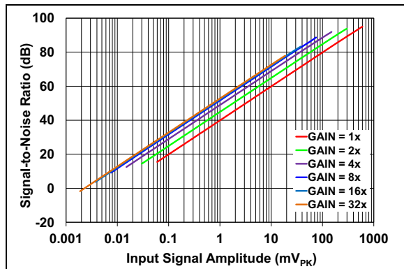
FIGURE 2-25: SNR vs. Input Signal Amplitude.
