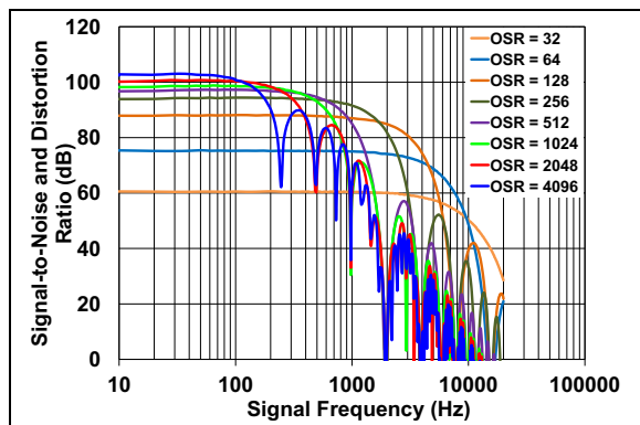
FIGURE 2-27: SINAD vs. Input Frequency.
