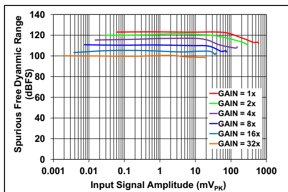
FIGURE 2-26: SFDR vs. Input Signal Amplitude.
