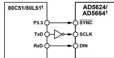
1 ADDITIONAL PINS OMITTED FOR CLARITY. 095943-040
