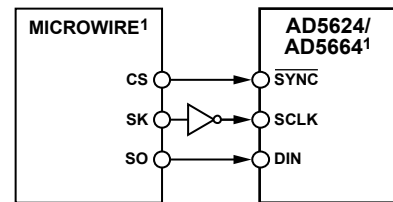
1 ADDITIONAL PINS OMITTED FOR CLARITY. 095943-041
