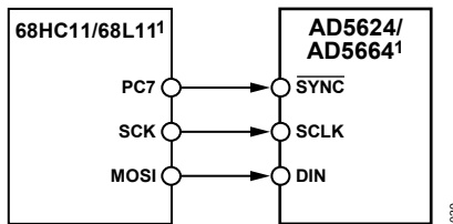
1 ADDITIONAL PINS OMITTED FOR CLARITY. 095943-039
