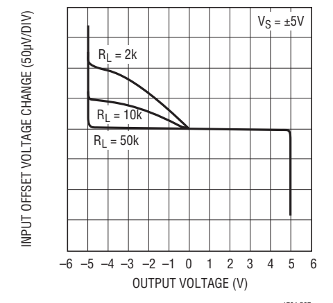
Open-Loop Gain
