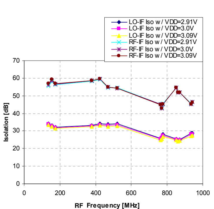
Figure 13. Isolation vs V_{DD}
