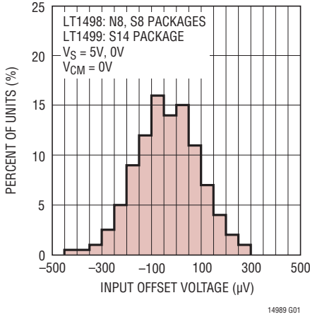
V_{OS} Distribution, V_{CM} = 0V (PNP Stage)
