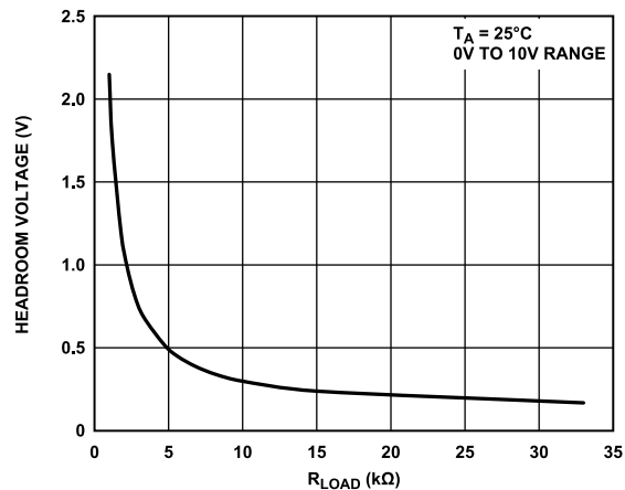
Figure 34. V_{OUT} Headroom
