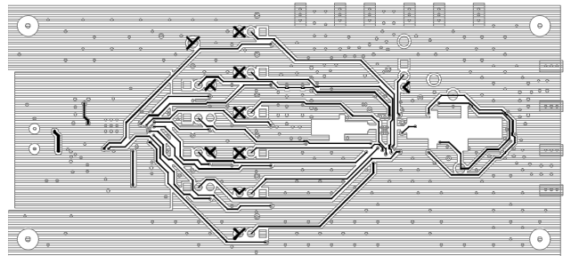
Figure 63. Bottom Layer
