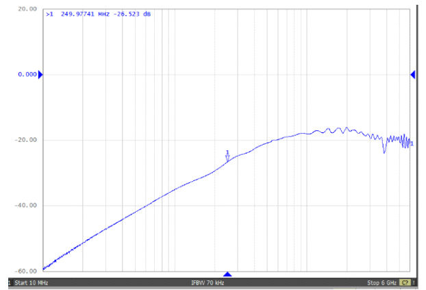
Figure 6-16. Off-State Data-Switch Isolation vs Frequency
