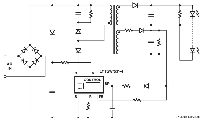
Figure 1. Typical Schematic.
