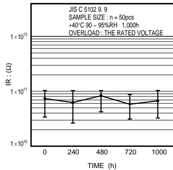
Fig.33 Insulation resistance
