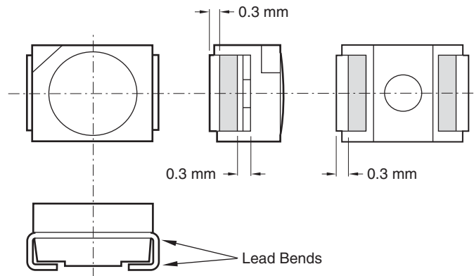
Fig. 9 Solderability Judgment Areas
