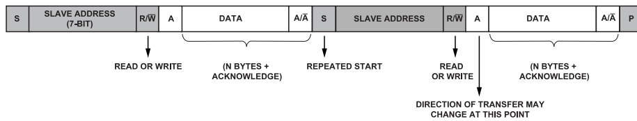
Figure 26. I 2 C—Combined Write/Read
