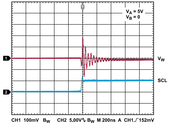
Figure 26. Digital Feedthrough
