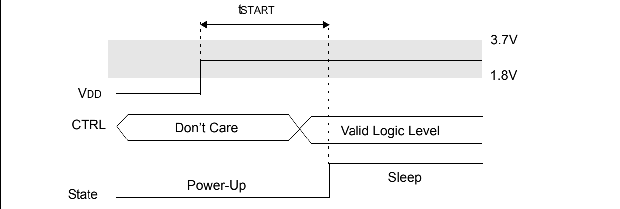
FIGURE 28-5: POWER-UP TIMING
