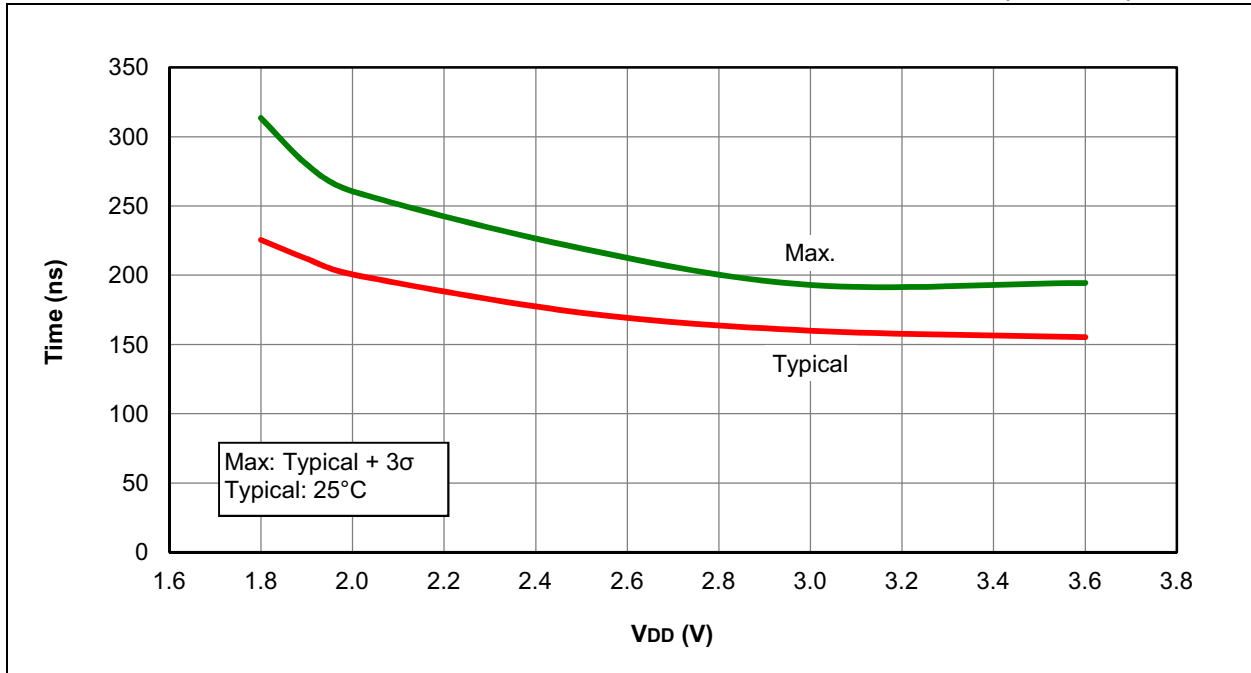
FIGURE 32-38: COMPARATOR RESPONSE TIME, NORMAL-POWER MODE (CxSP = 1)
