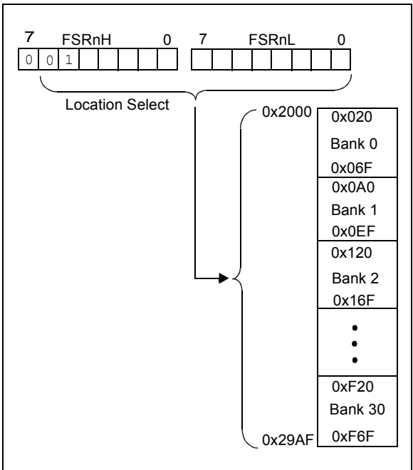
FIGURE 3-10: LINEAR DATA MEMORY MAP
