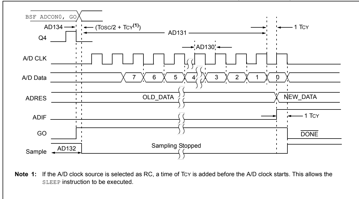
FIGURE 31-12: PIC12LF1840T48A A/D CONVERSION TIMING (SLEEP MODE)
