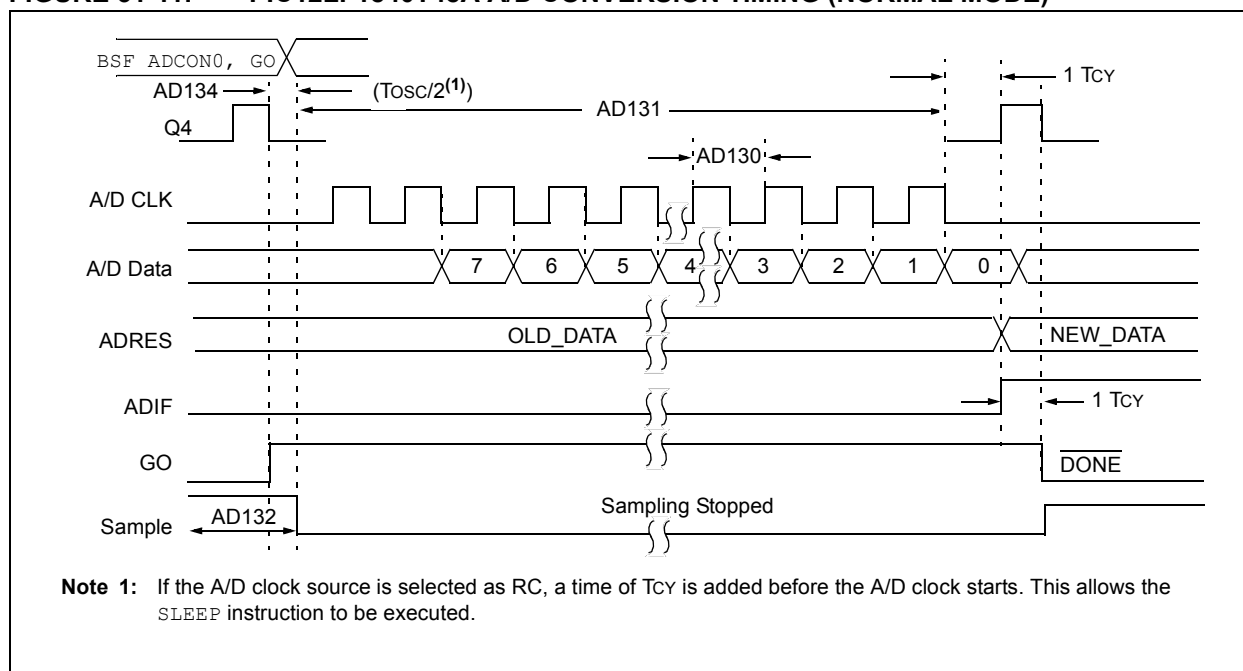
FIGURE 31-11: PIC12LF1840T48A A/D CONVERSION TIMING (NORMAL MODE)
