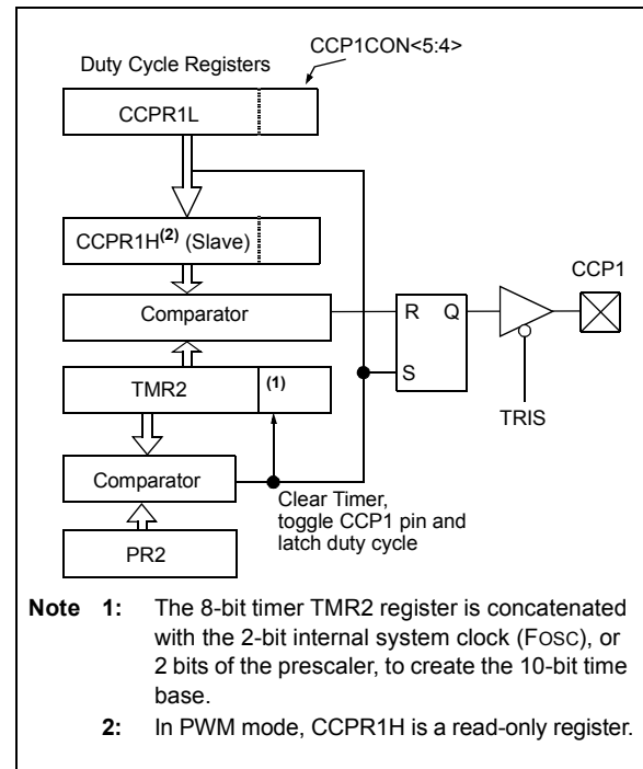
FIGURE 24-4: SIMPLIFIED PWM BLOCK DIAGRAM
