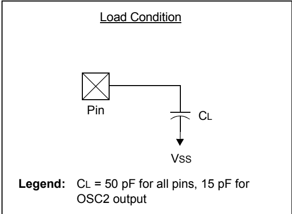
FIGURE 31-4: LOAD CONDITIONS
