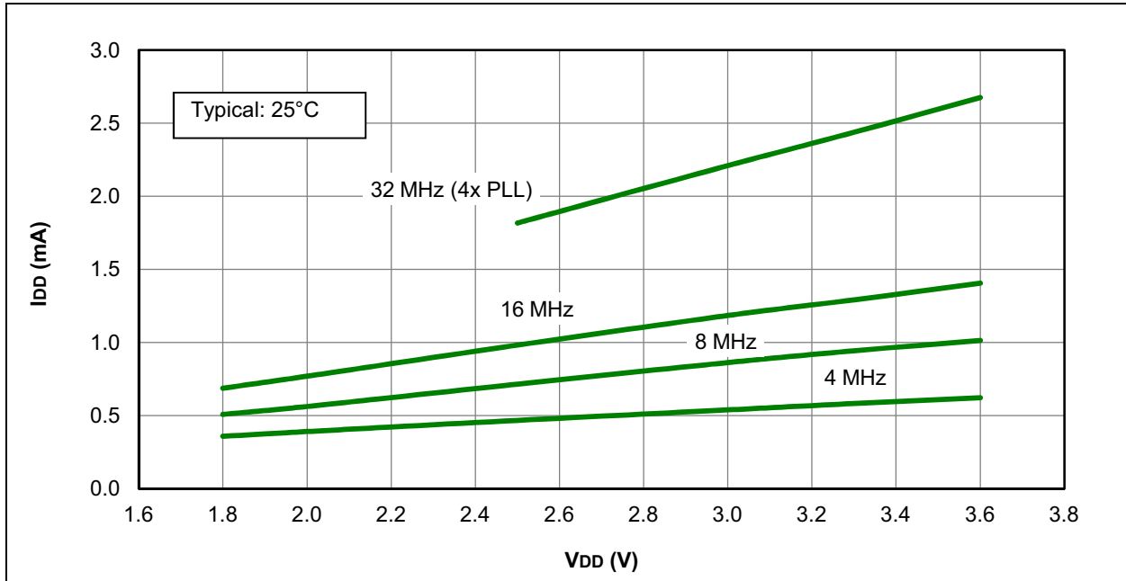
FIGURE 32-12: I DD TYPICAL, HFINTOSC
