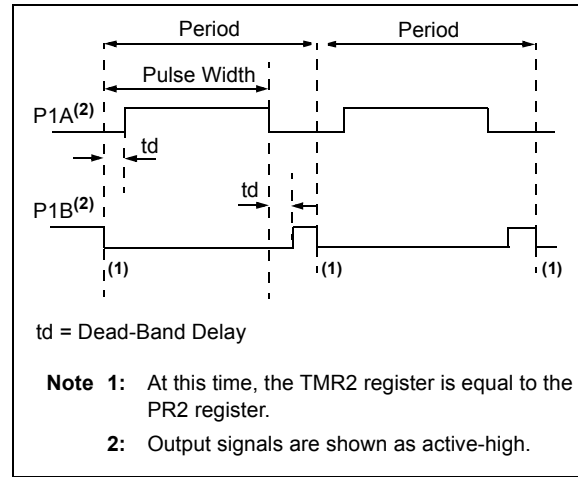
FIGURE 24-12: EXAMPLE OF HALF-BRIDGE PWM OUTPUT
