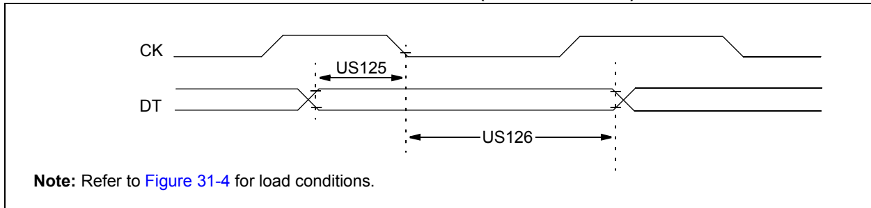
FIGURE 31-14: USART SYNCHRONOUS RECEIVE (MASTER/S�AVE) TIMING
