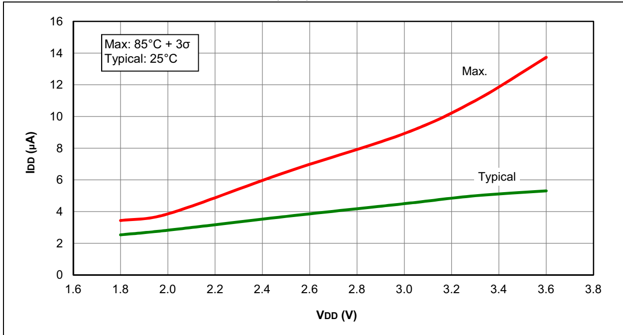
FIGURE 32-4: I_{DD} , EXTERNAL CLOCK (ECL), LOW-POWER MODE, F_{osc} = 32\text{ kHz}
