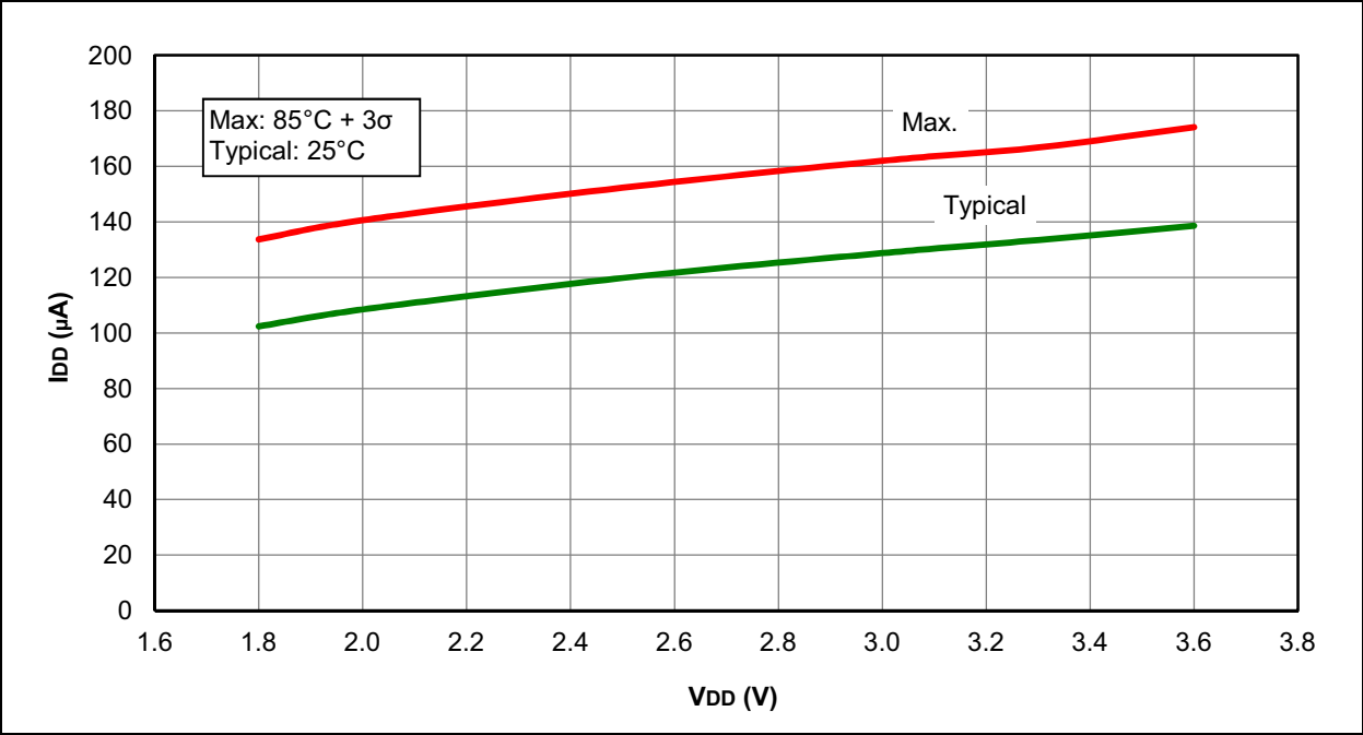
FIGURE 32-11: I_{DD} MFINTOSC, F_{osc} = 500\text{ kHz}
