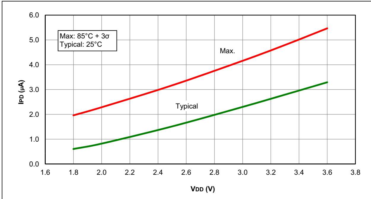
FIGURE 32-20: I_{PD} , SECONDARY OSCILLATOR, F_{osc} = 32\text{ kHz}
