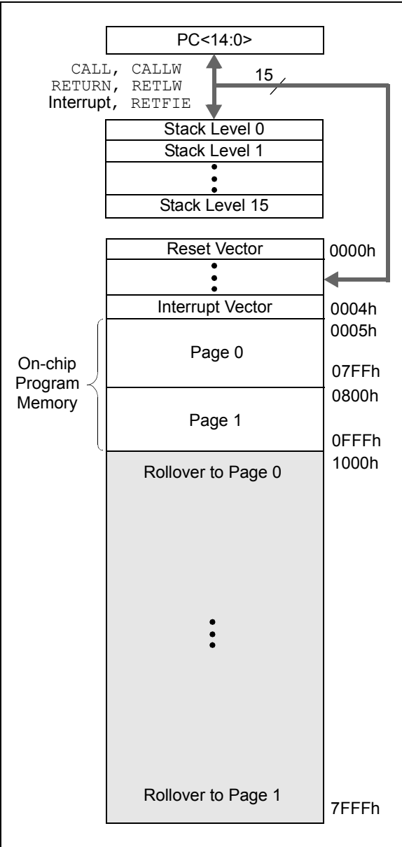
FIGURE 3-1: PROGRAM MEMORY MAP AND STACK FOR PIC12LF1840T48A
