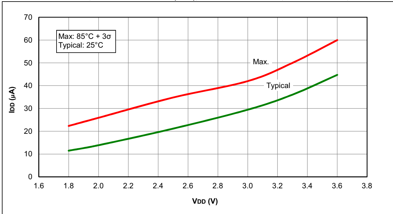
FIGURE 32-5: I_{DD} , EXTERNAL CLOCK (ECL), LOW-POWER MODE, F_{osc} = 500\text{ kHz} ,
