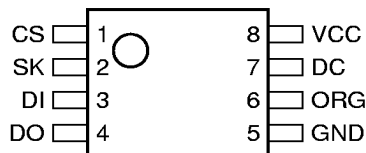
8-pin TSSOP
