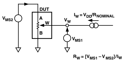
Figure 12. Wiper Resistance Test Circuit
