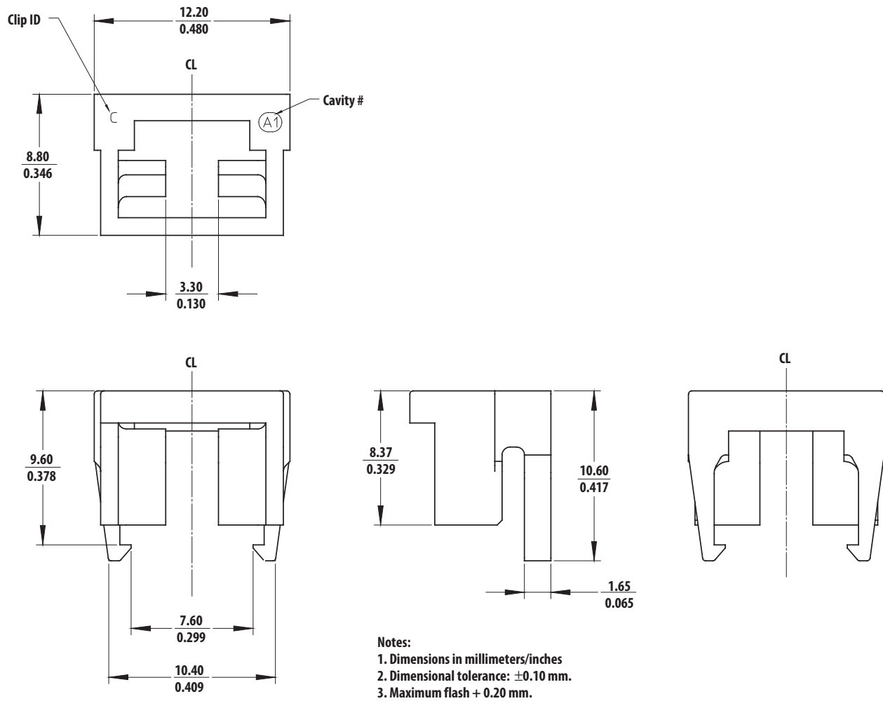
Figure 1. Outline Drawing for ADNS-6230-001 VCSEL Assembly Clip
