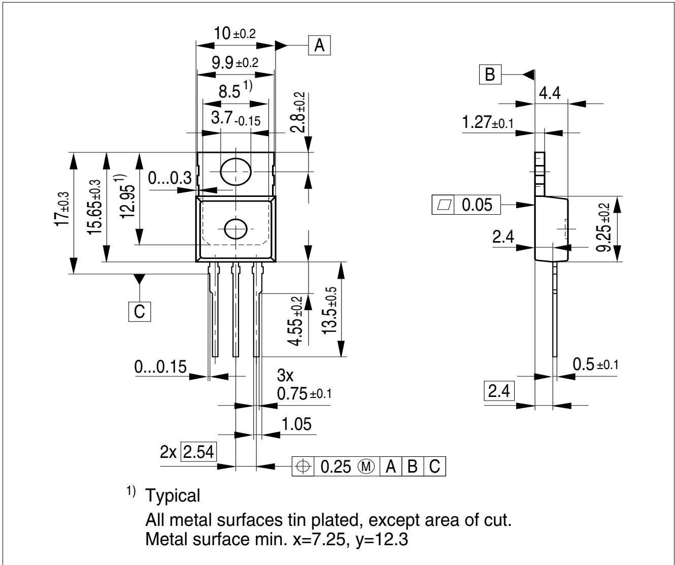
Figure 1 PG-TO220-3-1
