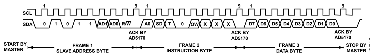
Figure 45. Writing Data to the RDAC Register
