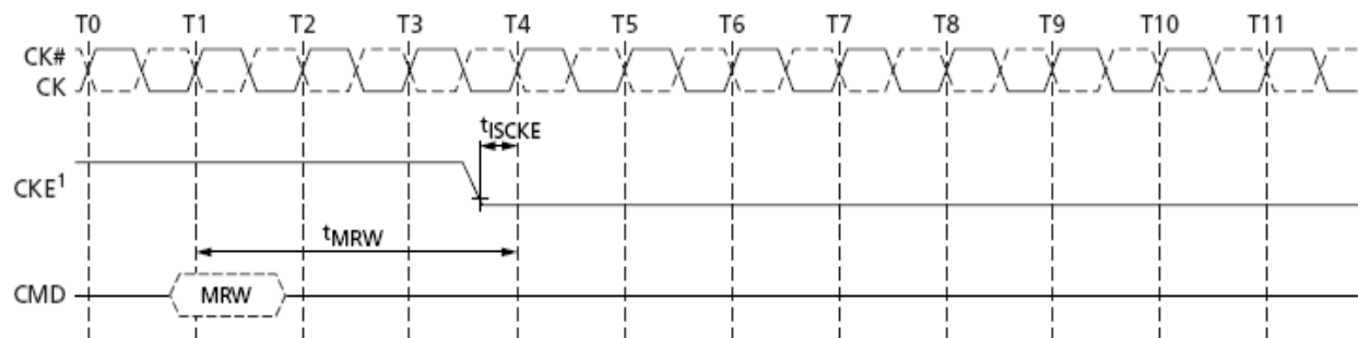
Mode Register Write to Power-Down entry
