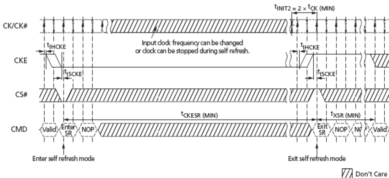
Self Refresh Operation
