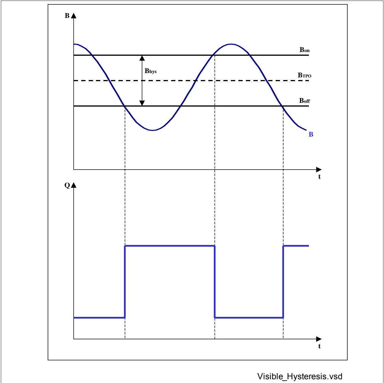
Figure 4 Visible Hysteresis
