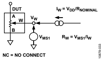
Figure 33. Wiper Resistance
