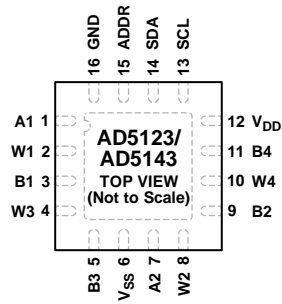
Figure 4. Pin Configuration
