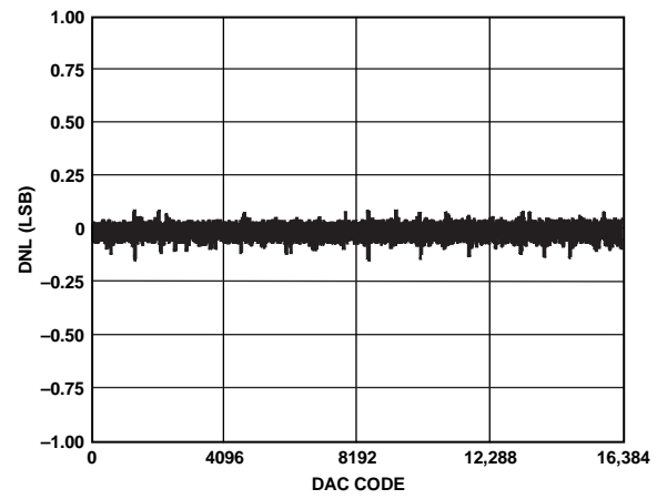
Figure 11. AD5025 DNL
