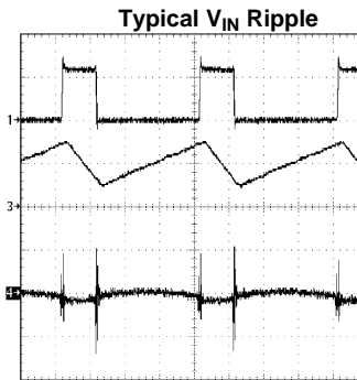
3 LEDs, R_{LED} = 22\Omega , V_{IN} = 3.0\text{V} , CNTRL = 2.7\text{V} 1) SW, 10 V/div, DC 3) I_L , 100 mA/div, DC 4) V_{IN} , 100 mV/div, AC T = 250 \text{ ns/div}
