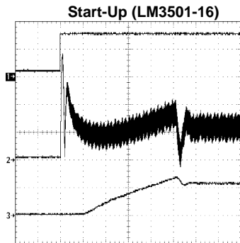
3 LEDs, R_{LED} = 22\Omega , V_{IN} = 3.0\text{V} , CNTRL = 2.7\text{V} 1) \overline{\text{SHDN}} , 1 V/div, DC 2) I_L , 100 mA/div, DC 3) I_{LED} , 20 mA/div, DC T = 100 \mu\text{s/div}
