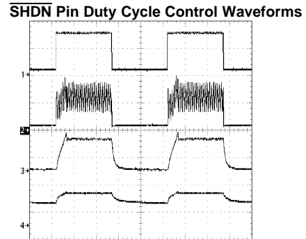
LM3501-16, 3 LEDs, R_{LED} = 22\Omega , V_{IN} = 3.0\text{V} , \overline{\text{SHDN}} frequency = 200 Hz 1) \overline{\text{SHDN}} , 1 V/div, DC 2) I_L , 100 mA/div, DC 3) I_{LED} , 20 mA/div, DC 4) V_{OUT} , 10 V/div, DC T = 1 \text{ ms/div}
