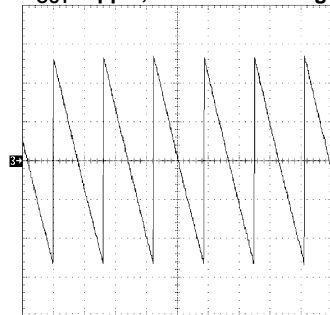
V_{OUT} open circuit and equals approximately 15V DC, V_{IN} = 3.0\text{V} 3) V_{OUT} , 200 mV/div, AC T = 1 \text{ ms/div}
