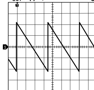
V_{OUT} open circuit and equals approximately 20V DC, V_{IN} = 3.0\text{V} 1) V_{OUT} , 200 mV/div, AC T = 400 \mu\text{s/div}
