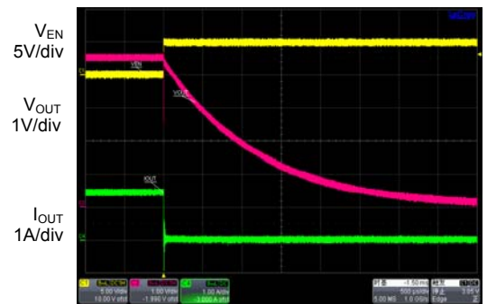
Time 500µs/div
