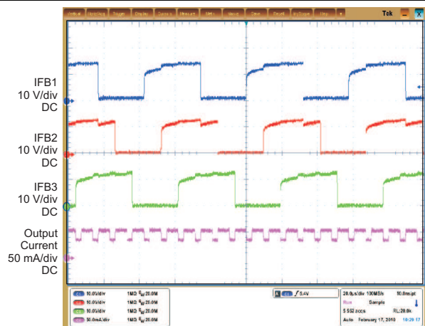
Figure 5. Switch Waveform
