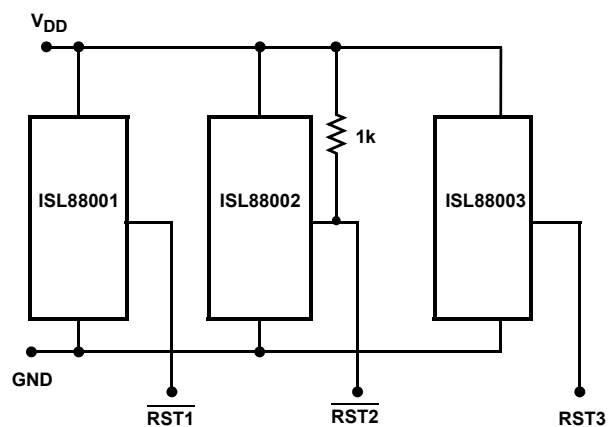
FIGURE 13. ISL88001/2/3EVAL1Z SCHEMATIC
