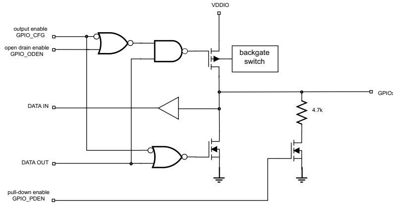
Figure 5-2. GPIO block
