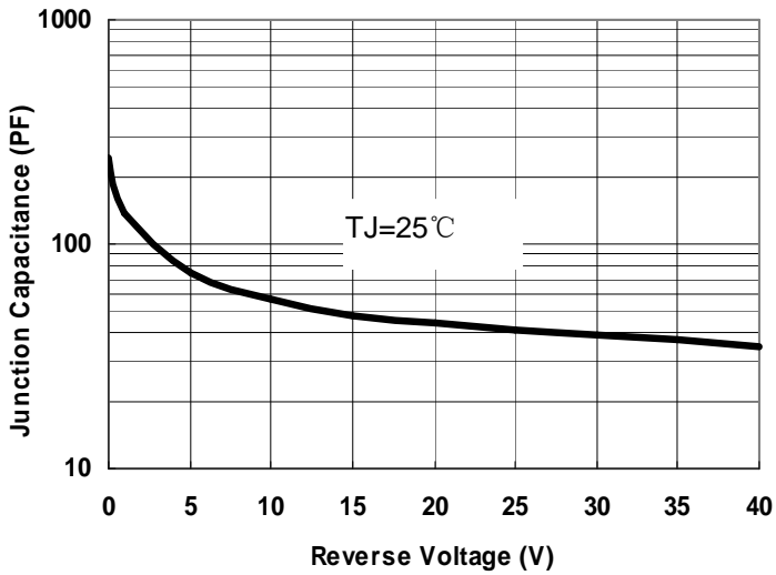
Fig.1-Typical Junction Capacitance
