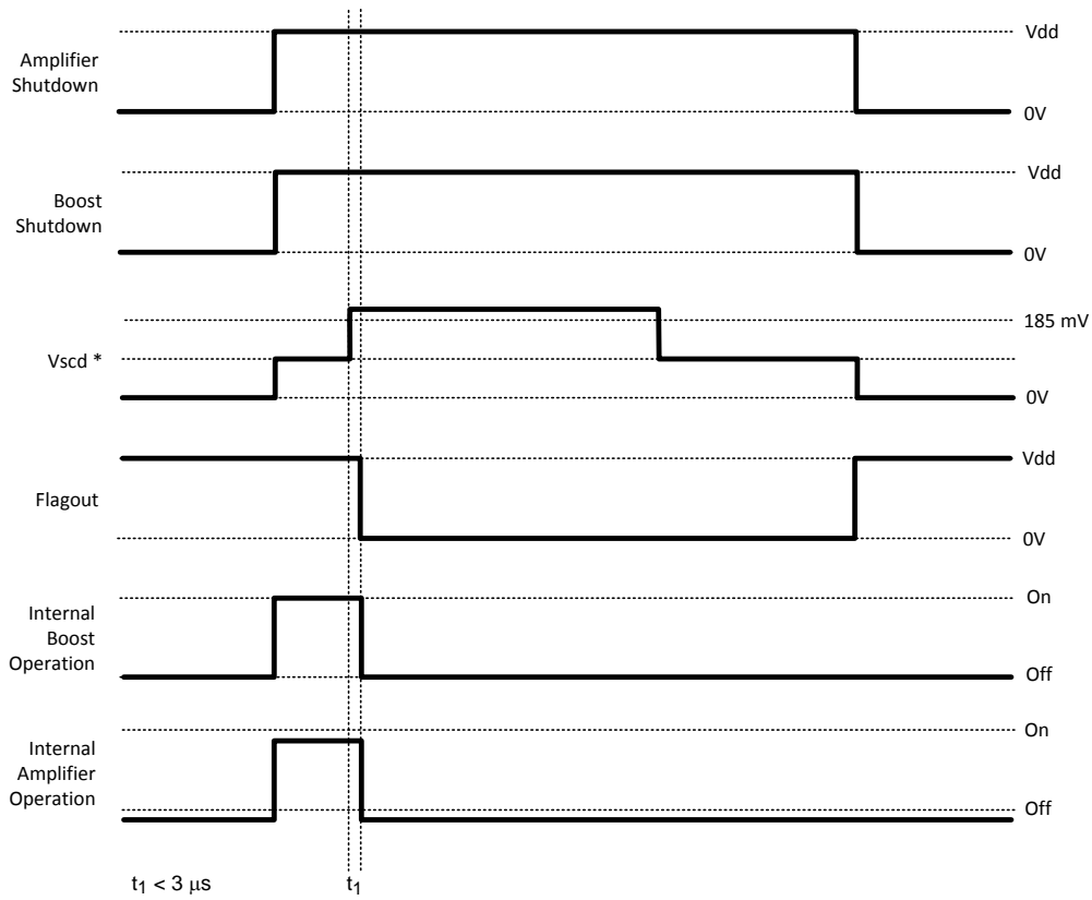
Figure 21. OCP Timing Diagram
