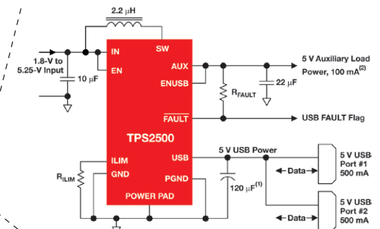
TPS2500 application diagram.
