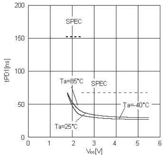
Figure 23. Data output delay time t_{PD1} ( CL=100\text{pF} )
