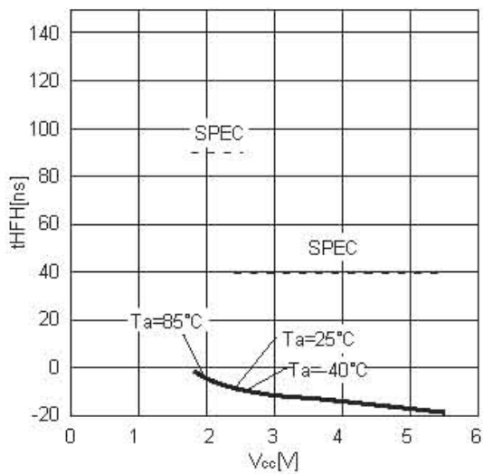
Figure 26. \overline{\text{HOLD}} setting hold time t_{HFH}
