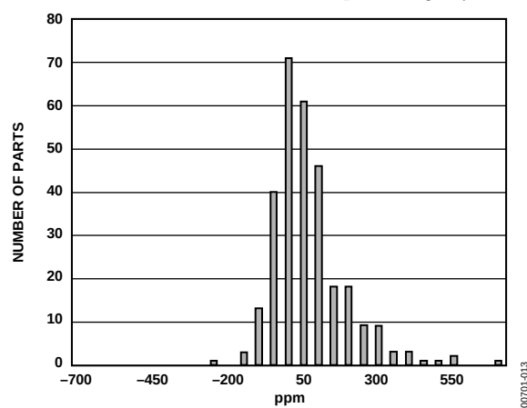
Figure 13. Output Voltage Hysteresis Distribution
