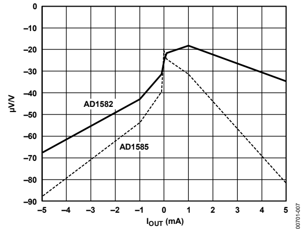
Figure 7. Line Regulation vs. I_{OUT}
