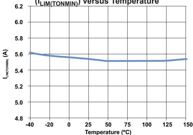
(I LIM(TONMIN) ) versus Temperature
