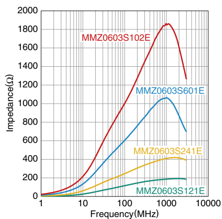
MMZ0603S-E series
