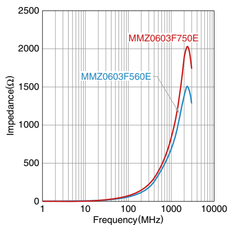
MMZ0603F-E series
