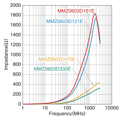
MMZ0603D-E series
