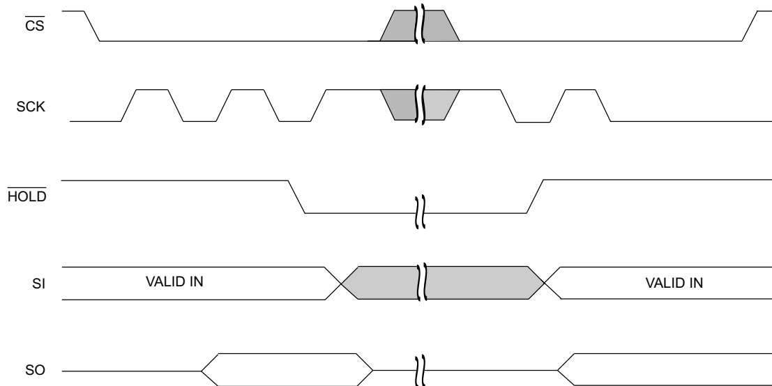
Figure 12. \overline{\text{HOLD}} Operation [2]
